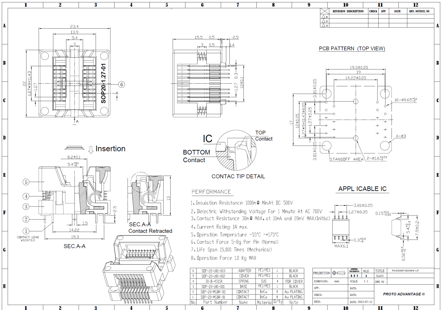
Image 3: Proto-Advantage PA-SOCKET-SOICW-8-1.27 Socket Drawing
