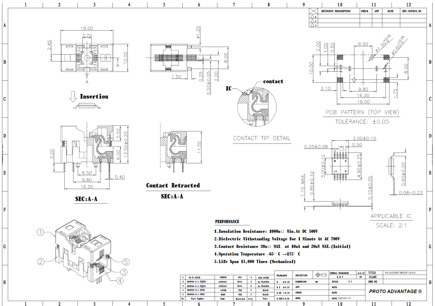
Image 3: Proto-Advantage PA-SOCKET-MSOP-10-0.5 Socket Drawing
