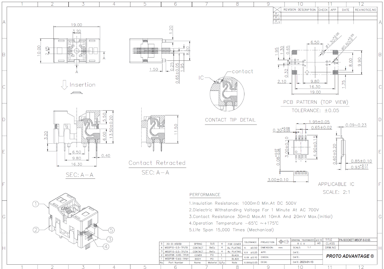
Image 3: Proto-Advantage PA-SOCKET-MSOP-8-0.65 Socket Drawing
